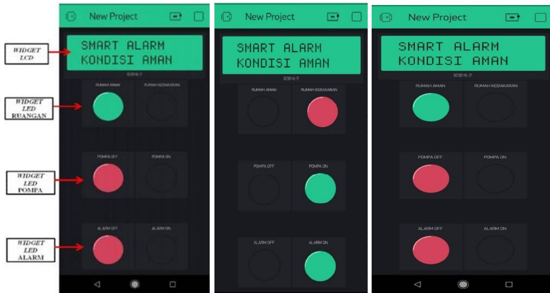
Figure 9. Blynk
