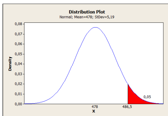
Gambar 24. Distribusi Plot Proses Coating
