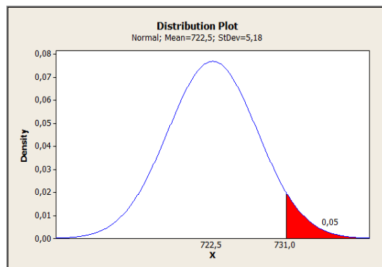
Gambar 20. Distribusi Plot Proses Welding 1
