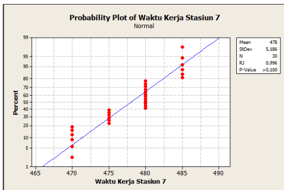
Gambar 23. Probability Plot Proses Coating
