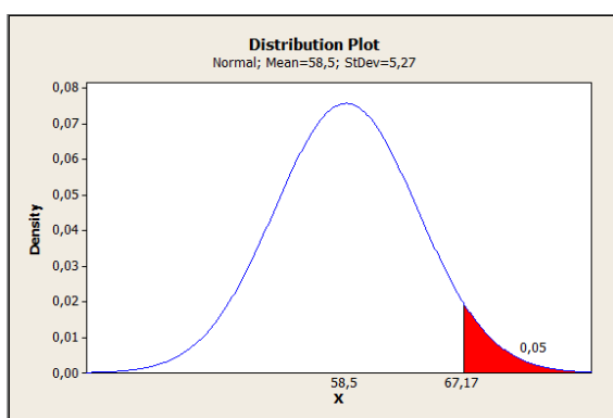
Gambar 16. Distribusi Plot Proses Bending
