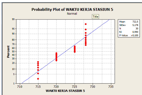
Gambar 19. Probability Plot Proses Welding 1
