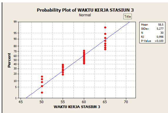
Gambar 15. Probability Plot Proses Bending
