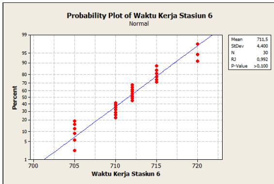
Gambar 21. Probability Plot Proses Welding 2
