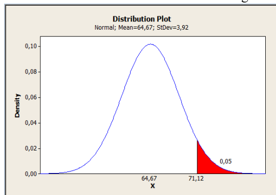
Gambar 18. Distribusi Plot Proses Bending Roll
